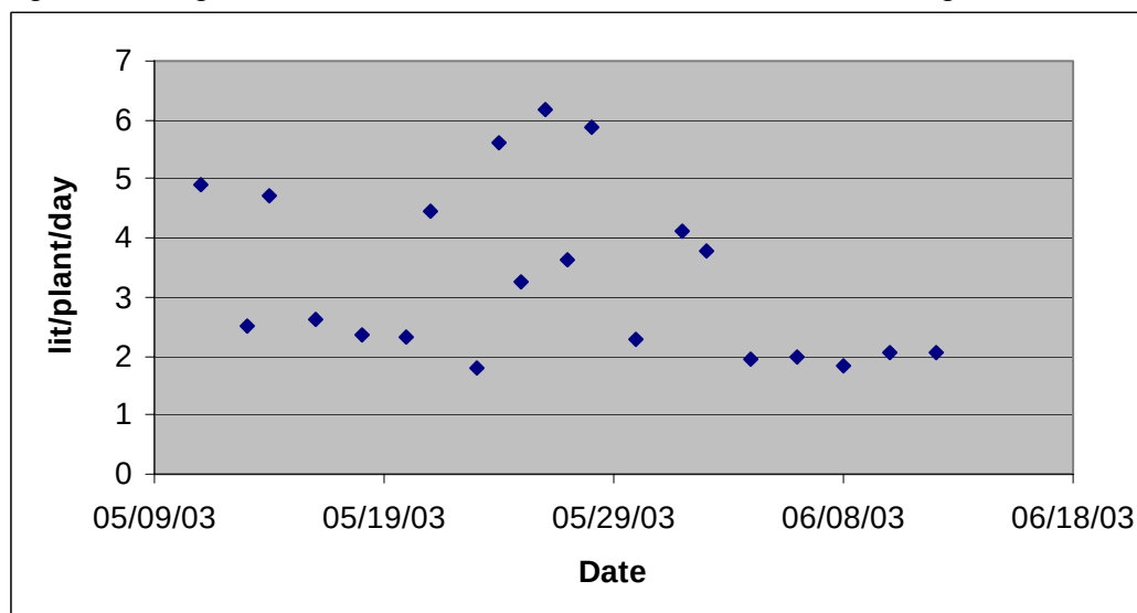
Figure 12: Irrigation Pattern for Pre-Monsoon Furrow Cotton during summer
