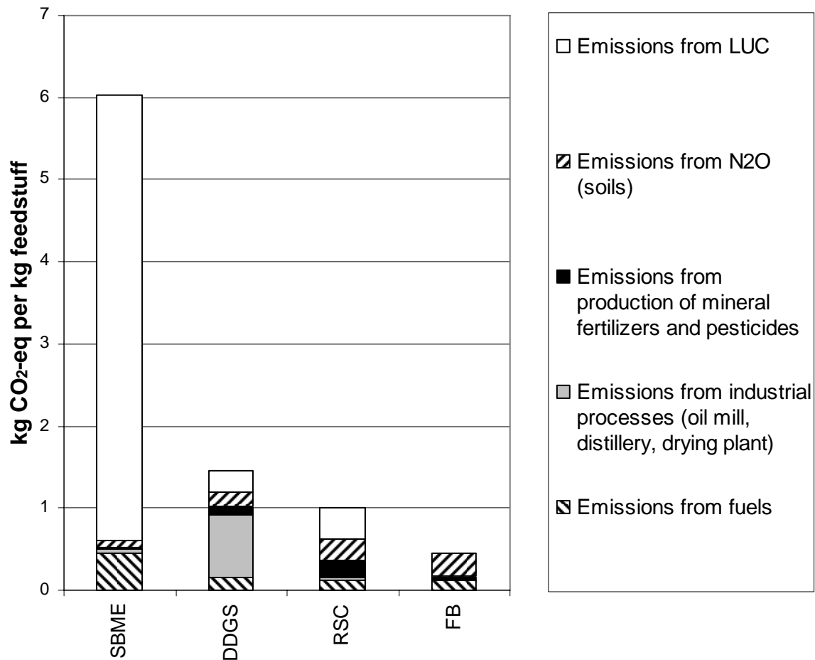
Figure 1. GHGE per kg of protein-rich feedstuffs (kg CO 2 -eq per kg DM feedstuff).
